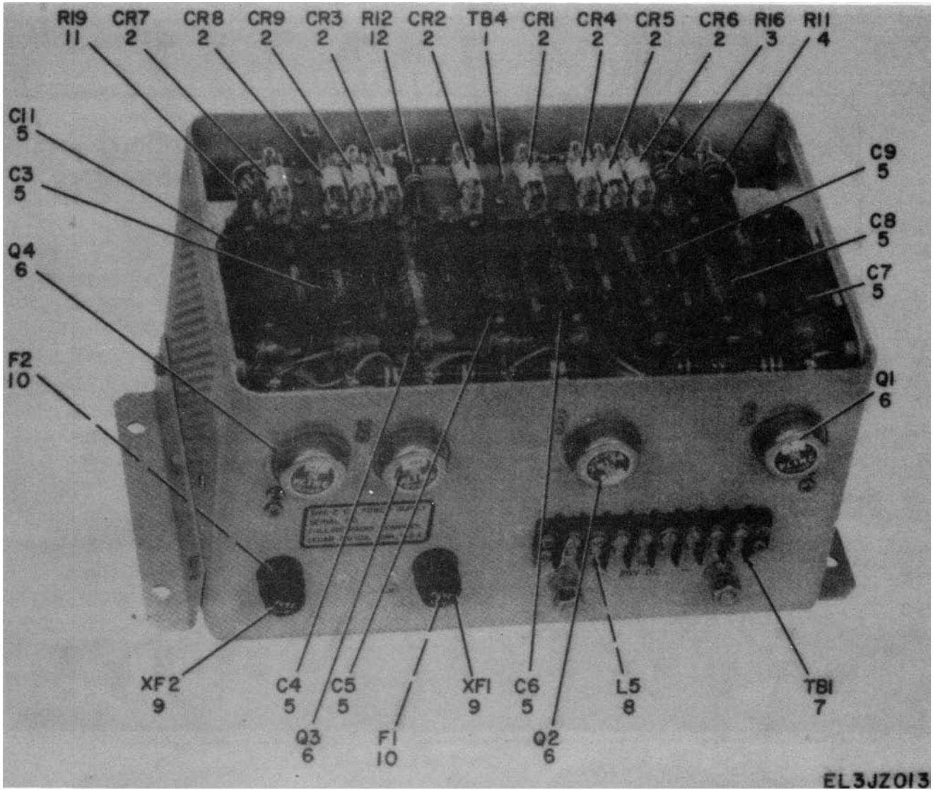
Figure 8. Power Supply PP-4765/GRC-159(V), Cover Removed (Sheet 1 of 2)
